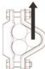
LATERAL LOAD 'HORIZONTAL DIRECTION'
